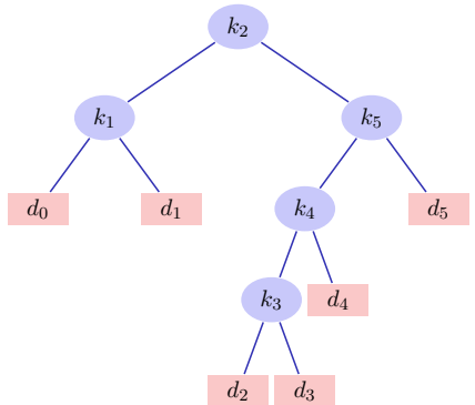
Search tree with expected costs 2.75
