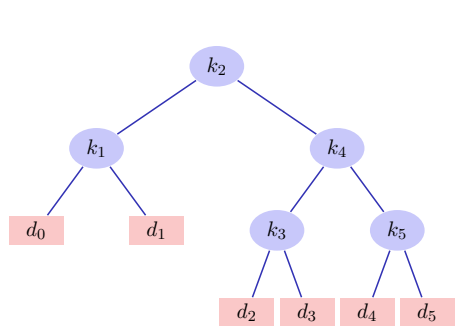
Search tree with expected costs 2.8
