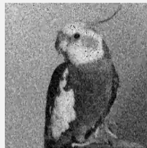
\gamma = 0.03
