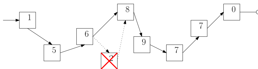
Figure 28: Removing node 2
